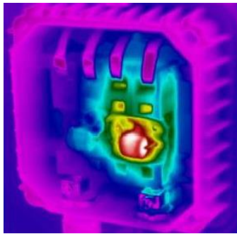
Figuur 36: oververhitte bypass-diode
